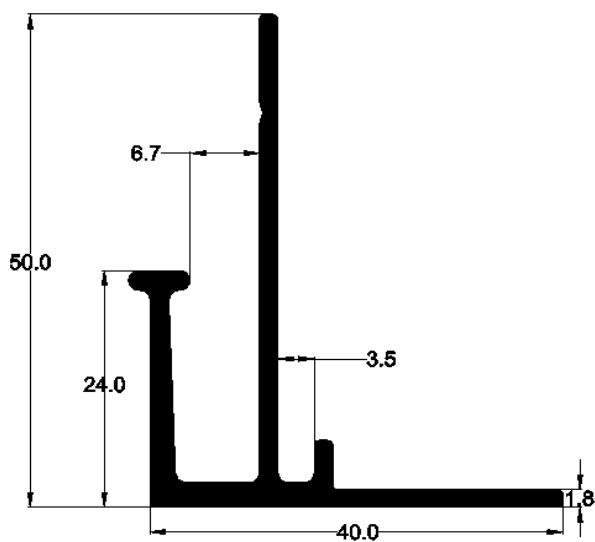
"F" PROFILE - AMS0414
