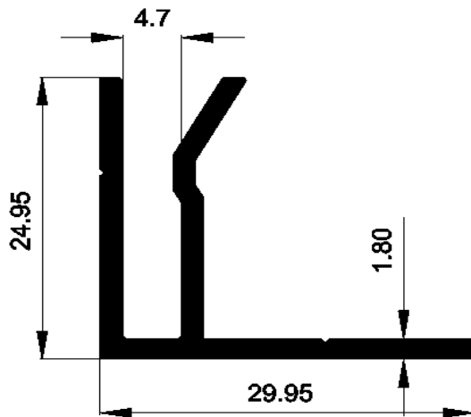
WINDOW FIXING - AMS0426
