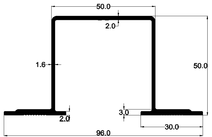
"U" PROFILE - AMS0415
