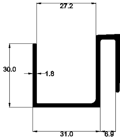
"S" PROFILE - AMS0412
