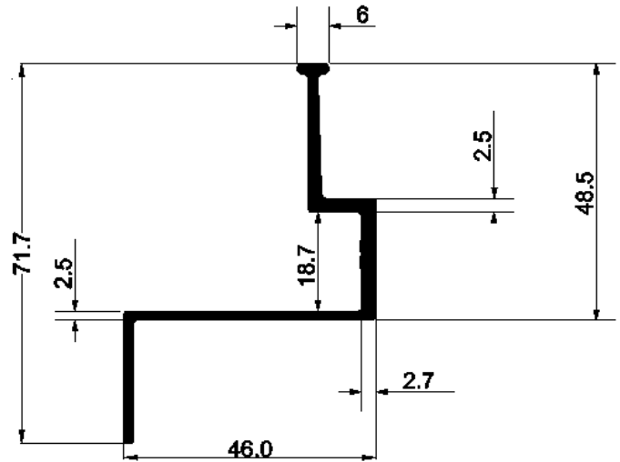
"Z" PROFILE - AMS0413
