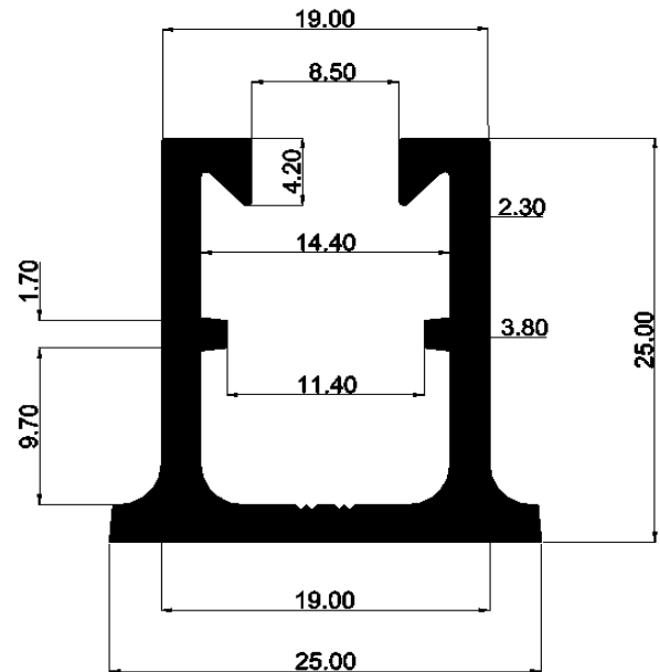
SIGN RAIL - AMS0227
