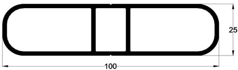
100mm GATE RAIL - AMS0451
